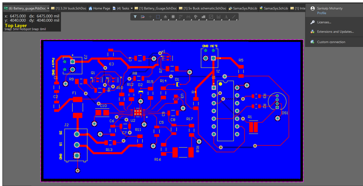
Layout of Fuel Gauge Battery Monitoring Board
