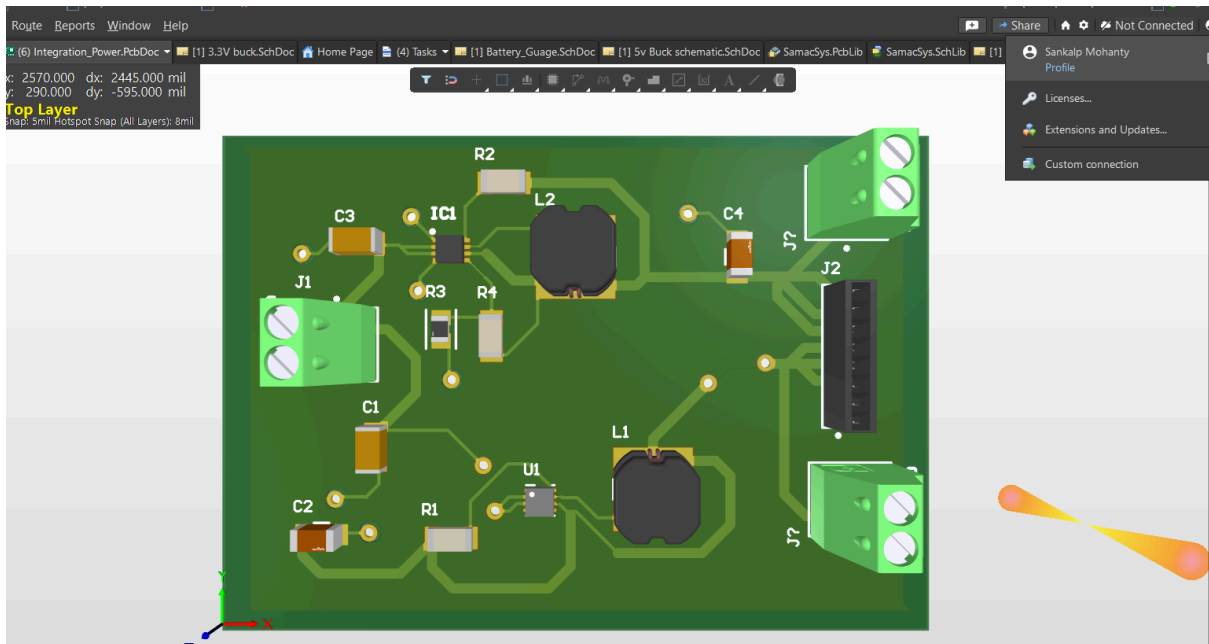
3.3V and 5V buck converter 3D View
