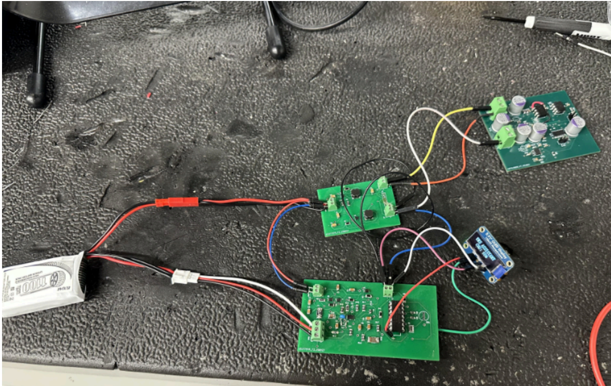
Pre-integration Battery Monitoring, buck converter, and data acquisition boards.
