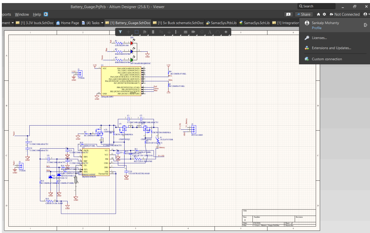
Fuel Gauge Battery Monitoring Schematic
