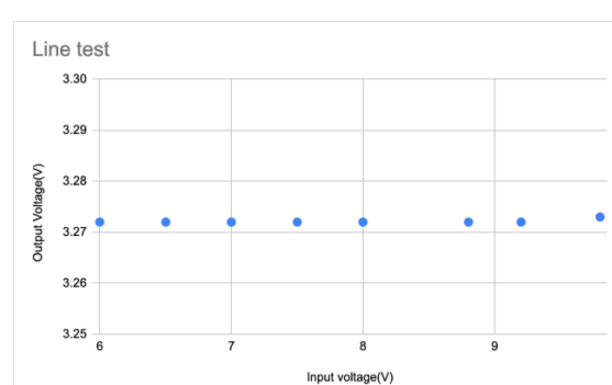
Line and Load tests for 3.3V buck converter, verified with an electronic load
