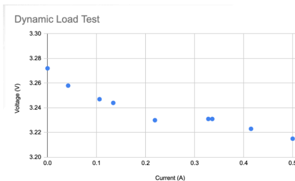
Line and Load tests for 3.3V buck converter, verified with an electronic load
