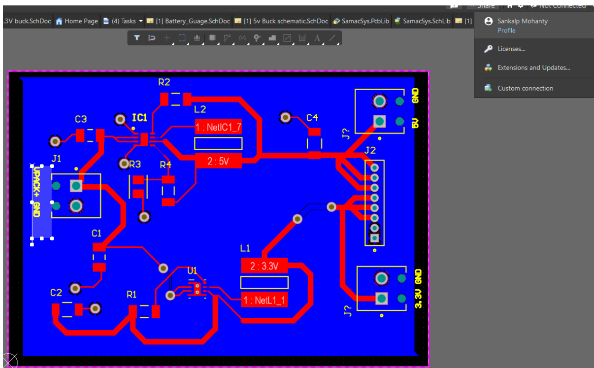
Layout of 3.3V and 5V buck converter Board
