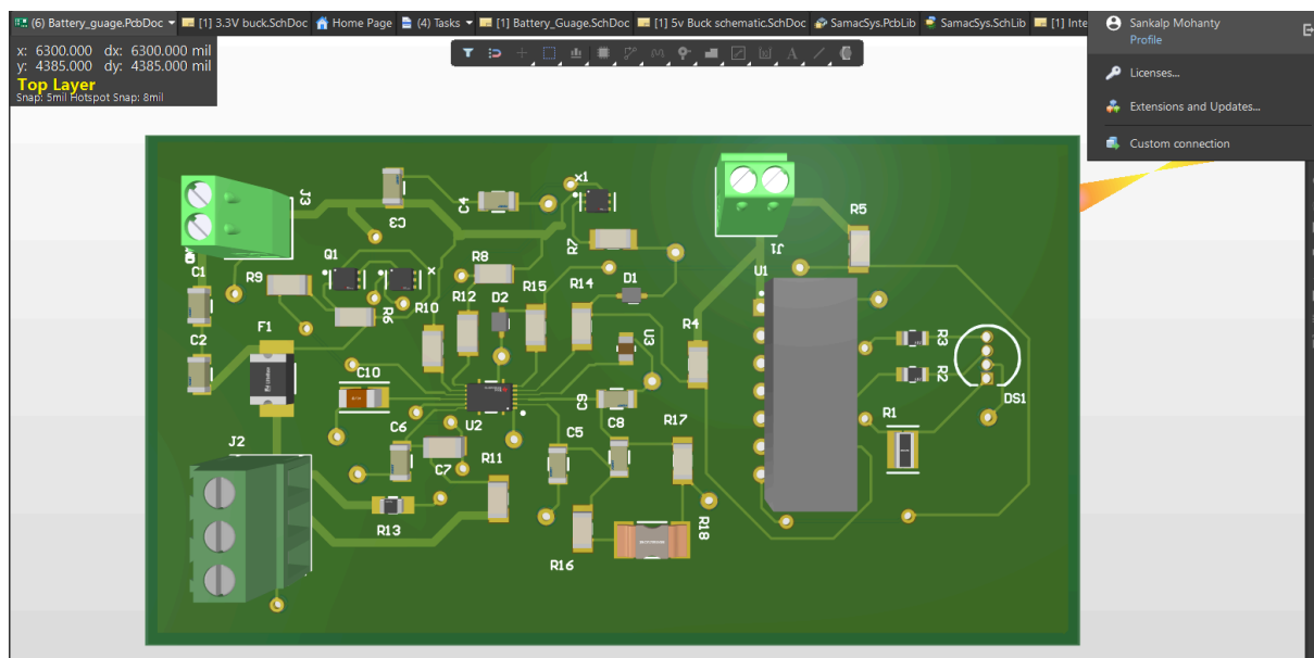
Fuel Gauge Battery Monitoring Board 3D View
